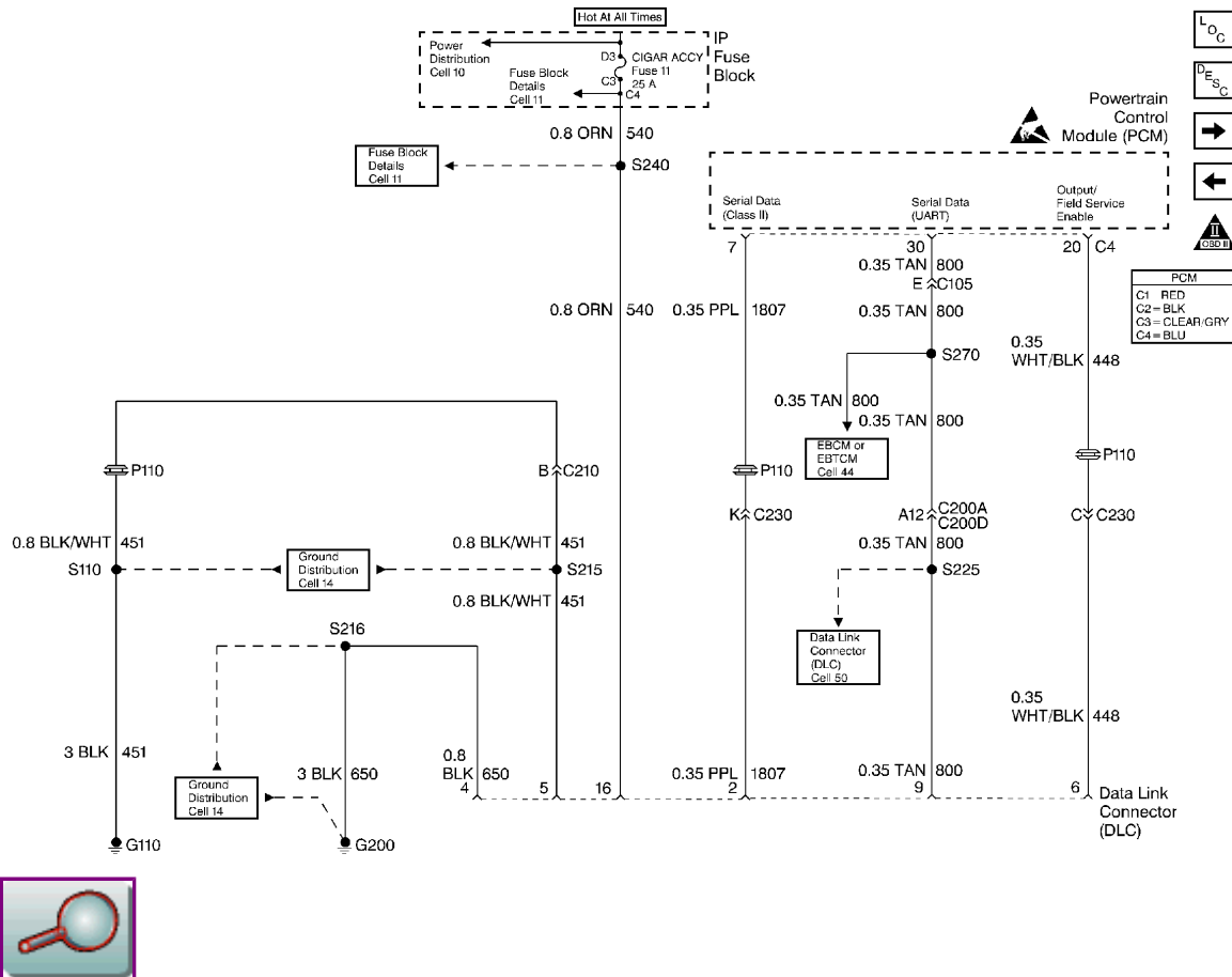
FIGURE Data Link Connector(c)
